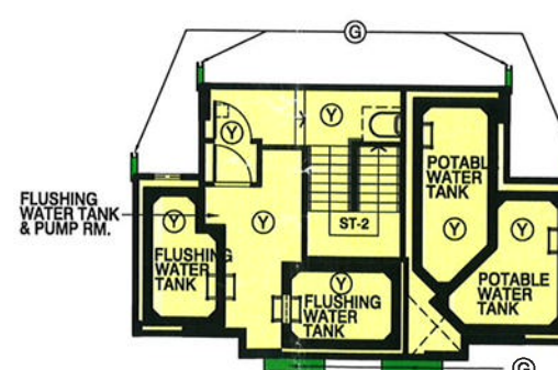
UPPER ROOF PLAN
